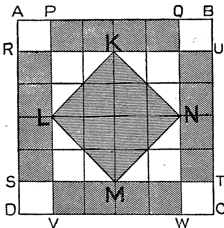
FIG. 14.—PROBLEM ON MAXIMA AND MINIMA (CASE I.),
